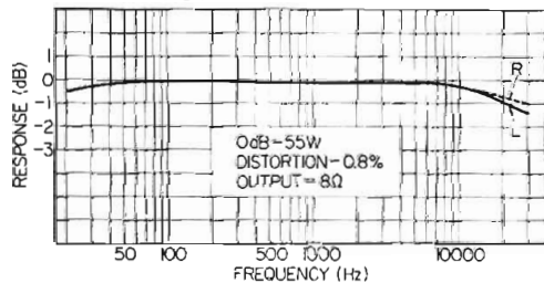
POWER BANDWIDTH
