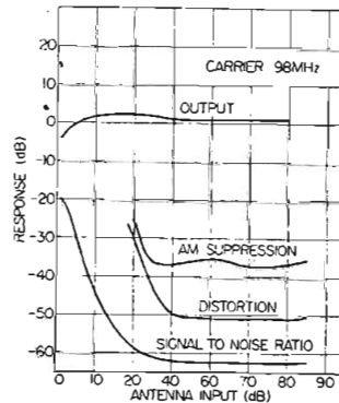
FM SIGNAL TO NOISE RATIO, OUTPUT LEVEL VS ANTENNA INPUT, DISTORTION & AMPLITUDE MODULATION SUPPRESSION RATIO
