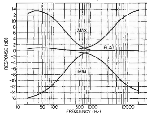
TONE CONTROL
