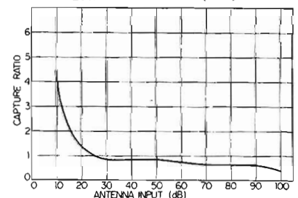
CAPTURE RATIO (IHF)
