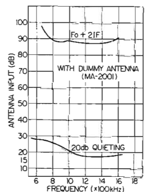
AM SENSITIVITY & IMAGE RATIO
